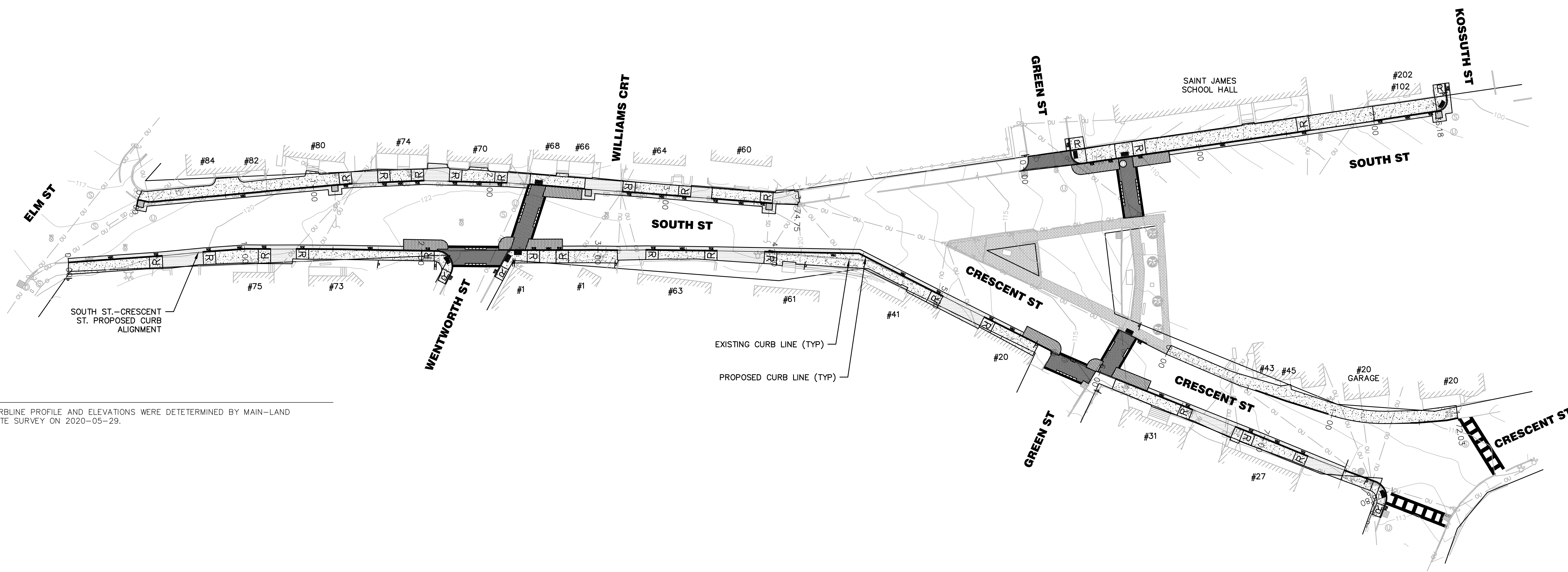
SOUTH ST.-CRESCENT ST. PLAN B1 HORIZONTAL SCALE 1" = 30'
