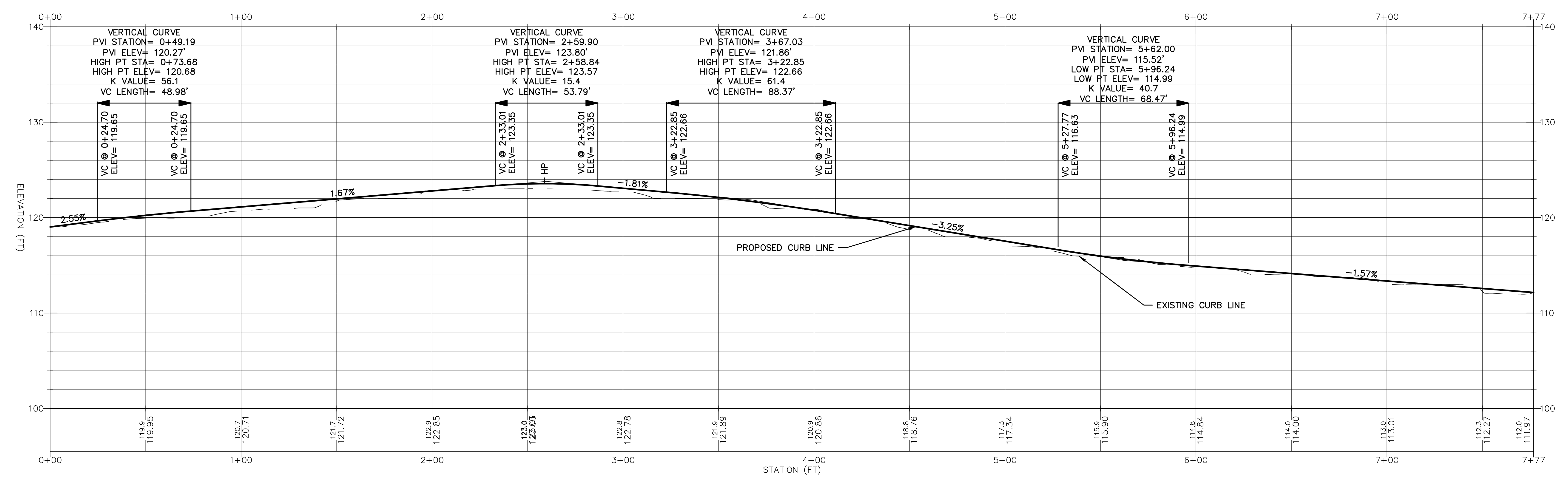
SOUTH ST.-CRESCENT ST. PROFILE A1 HORIZONTAL SCALE 1" = 30' VERTICAL SCALE 1" = 6'
